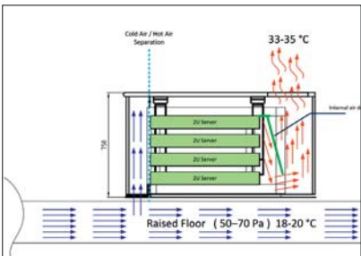
Cooling System
